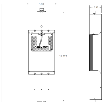
CEPS-125 with Grid Mount
