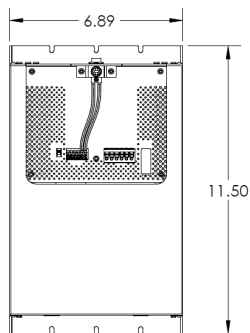
CEPS-125 only
