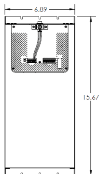
CEPS-250 only
