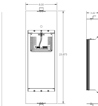
CEPS-250 with Grid Mount
